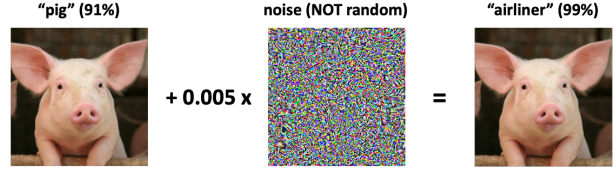
Figure 1. In the left picture, the network confidently predicts "pig" (91%). When combined with adversarial perturbation, the classifier is fooled, now predicting "airliner" (99%). Figure taken from Kolter & Madry (2018).
